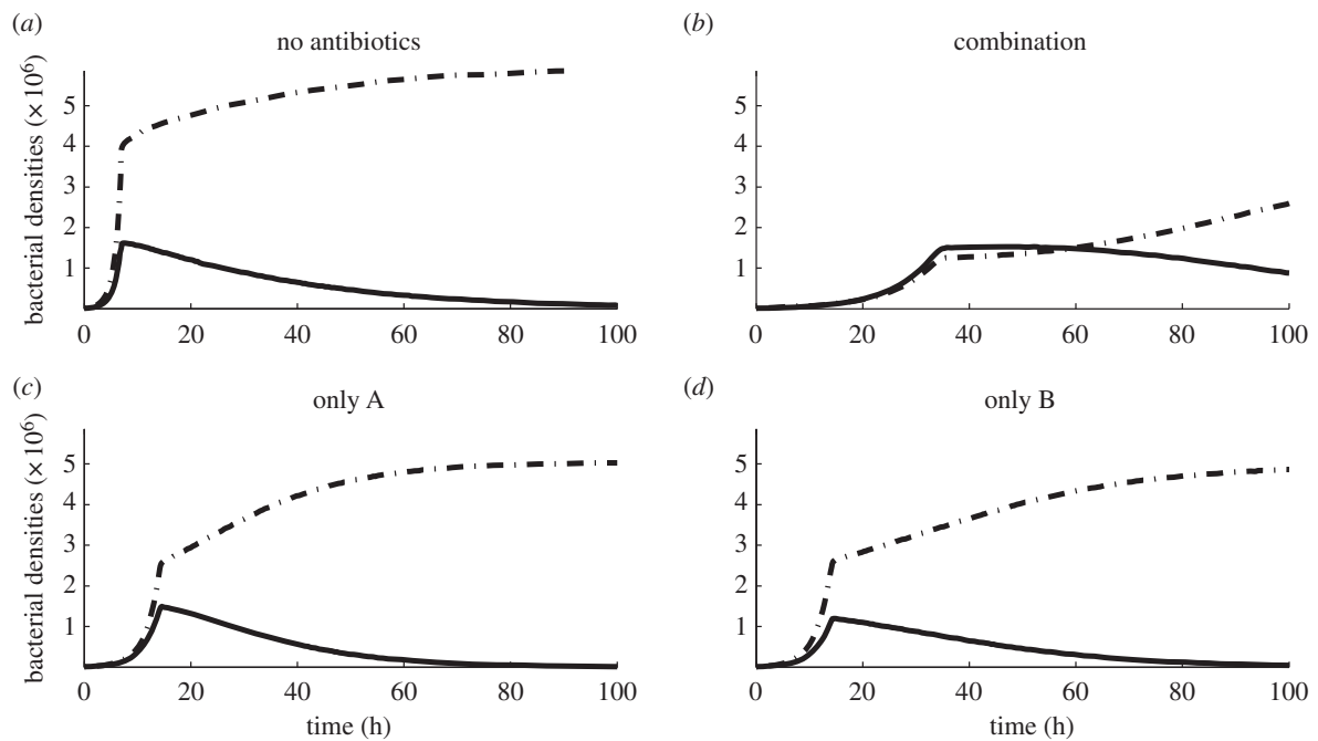
Figure 6. Numerical simulations with the parameter values given in table 1 showing the densities of pathogens (dashed-dotted lines) and commensals (solid lines) throughout an experiment of duration T = 100 h. (a) Bacterial densities (per millilitre) when no antibiotics are used and drug-susceptible pathogens colonize the system. (b) As the two antibiotics are synergistic, a 50–50 combination strategy (equal concentrations of each drug) is most effective at suppressing the density of pathogens. However, commensals are also suppressed, eventually allowing the multi-drug-resistant pathogen to colonize the host. (c,d) Single-drug protocols are ineffective, allowing resistant pathogens to colonize the system.
